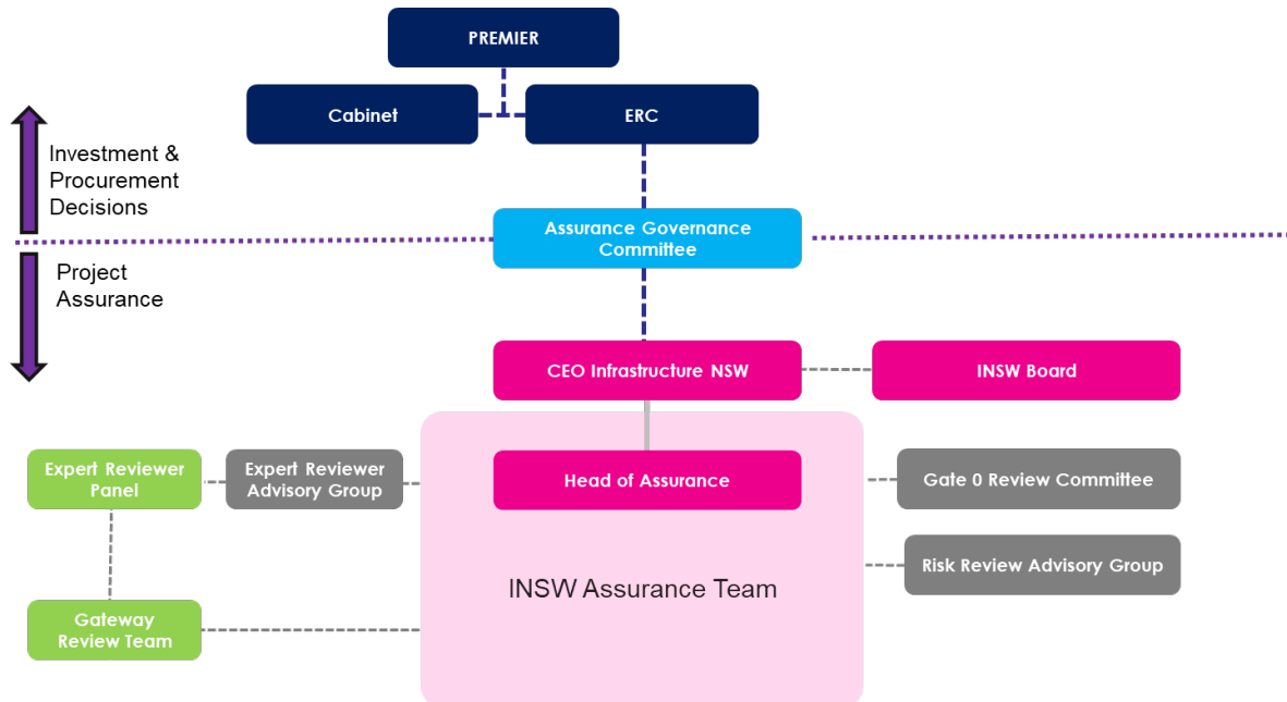
Figure 2 Framework Governance
